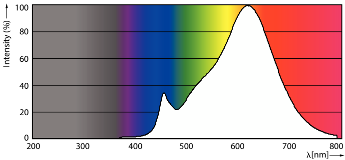
Spectral Power Distribution Colour - 3.3B11/PER/927-922/CL/G/E26/WGX1FB T20
