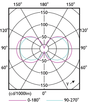
Light Distribution Diagram - 3.3B11/PER/927-922/CL/G/E26/WGX1FB T20
