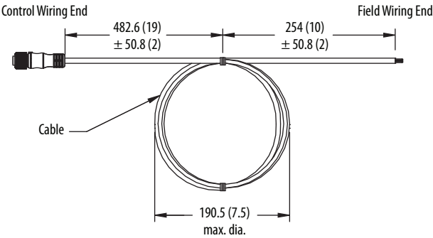
Cable Coiling
