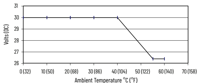
Maximum Output Voltage - 24V DC Operation
