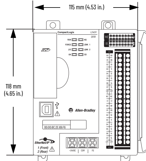
1769-L24ER-QBFC1B, 1769-L24ER-QBFC1BK, 1769-L27ERM-QBFC1B
