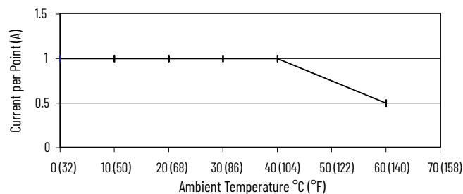
Maximum Input Current Per Point - 5V DC Operation
