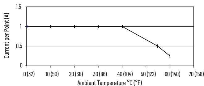
Maximum Output Current Per Point - 24V DC Operation
