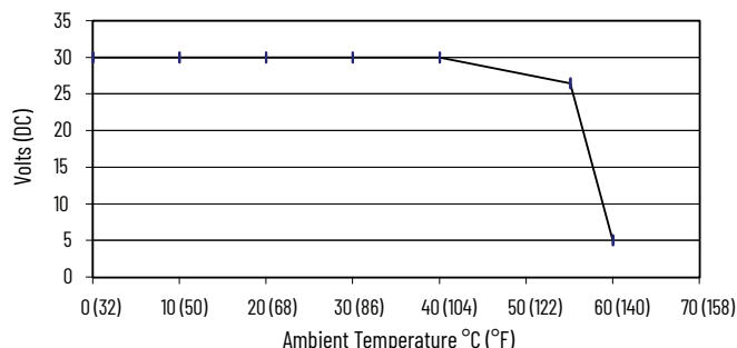
Maximum Input Voltage - 24V DC Operation
