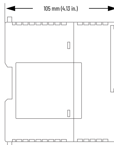
All CompactLogix 5370 L2 Controllers Side View
