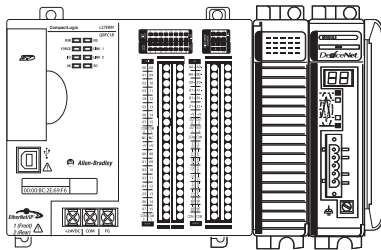
CompactLogix 5370 L3 Control System
