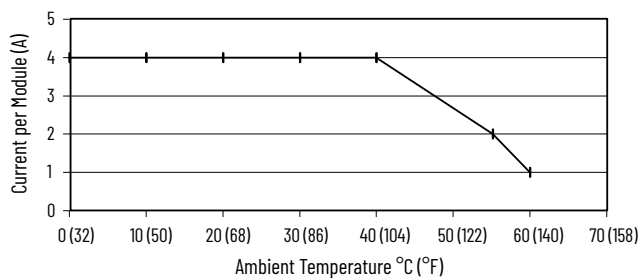
Maximum Output Current Per Module - 24V DC Operation
