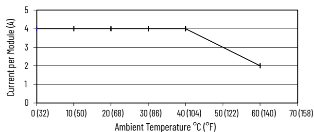
Maximum Output Current Per Point - 5V DC Operation
