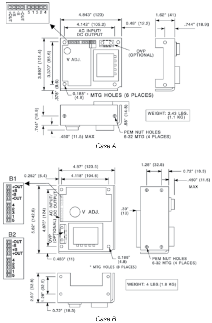
Dimensions - inches (mm)
