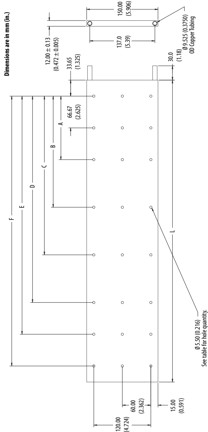
LDC-150-xxx-CP Motor Coil Cooling Plate Dimensions
