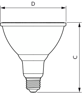
13PAR38/LED/940/F25/DIM/GULW/T20 6/1FB
