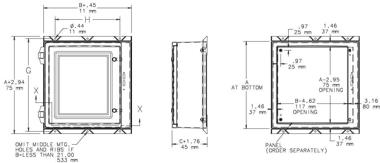
FRONT VIEW WITH DOOR SIDE VIEW FRONT VIEW DOOR REMOVED
