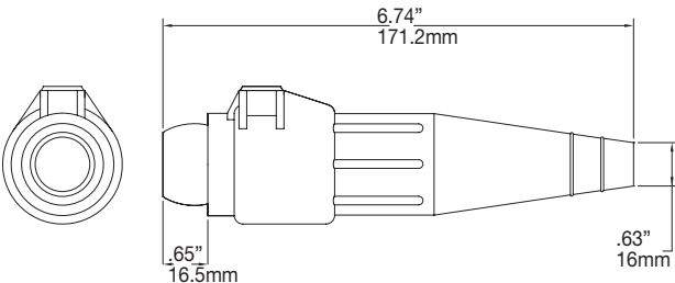
Female connector
