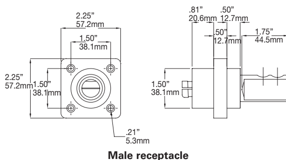
Male receptacle
