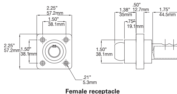
Female receptacle
