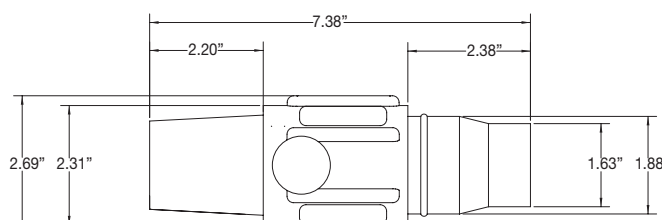
Female connector
