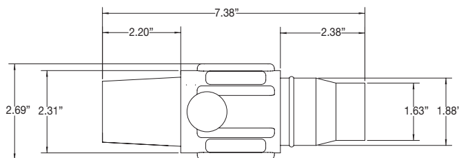
Female connector
