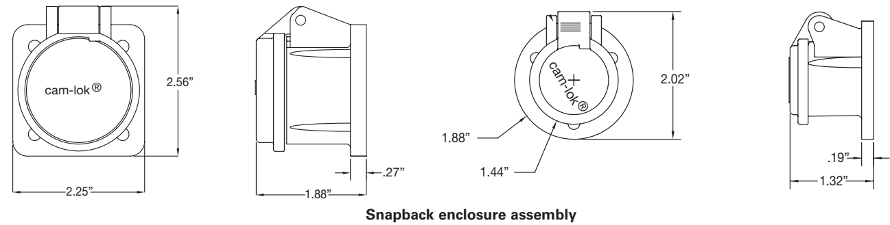
Snapback enclosure assembly
