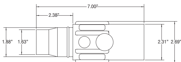
Male connector
