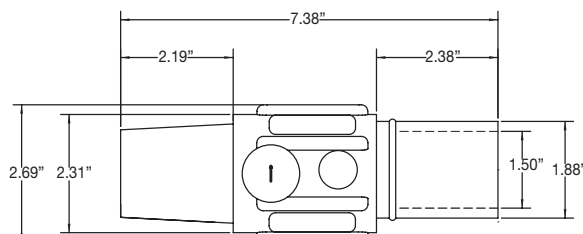
Female connector
