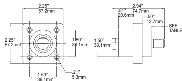
Male receptacle
