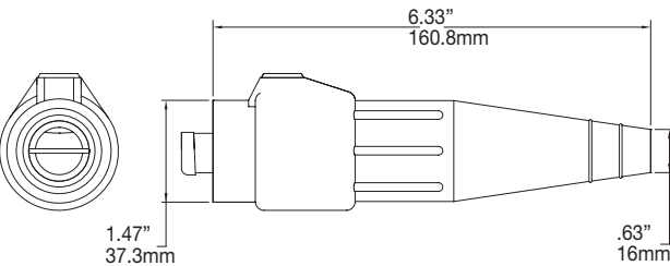
Male connector
