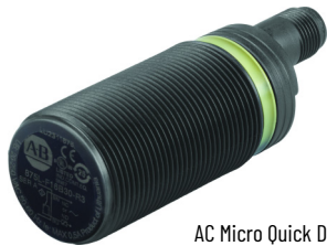
AC Micro Quick Disconnect Style 18 mm and 30 mm Shielded and Unshielded
