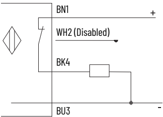
Figure 9 - Sourcing N.C.
