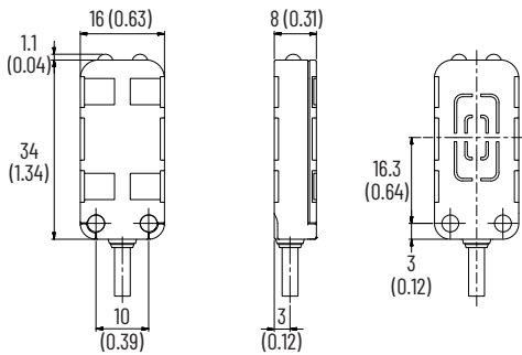
Figure 24 - Sensor
