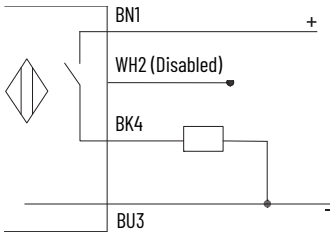
Figure 10 - Sourcing N.O.
