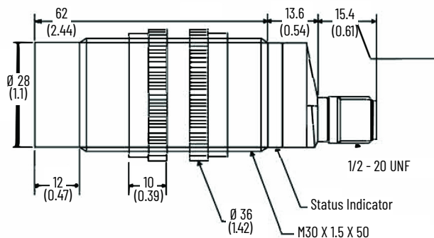
Figure 20 - AC Unshielded 30 mm (1.81 in.) with AC Micro QD [mm (in.)]
