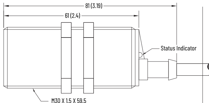
Figure 7 - Unshielded 30 mm (1.81 in.) with Cable [mm (in.)]
