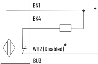
Figure 11 - Sinking N.C.
