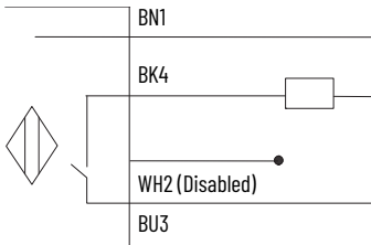
Figure 12 - Sinking N.O.
