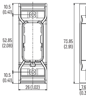
Figure 25 - Mounting Bracket
