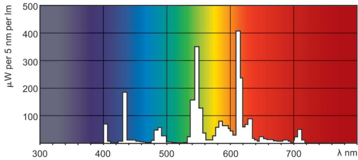
Spectral Power Distribution Colour - PL-L 36W/830/4P 1CT/25
