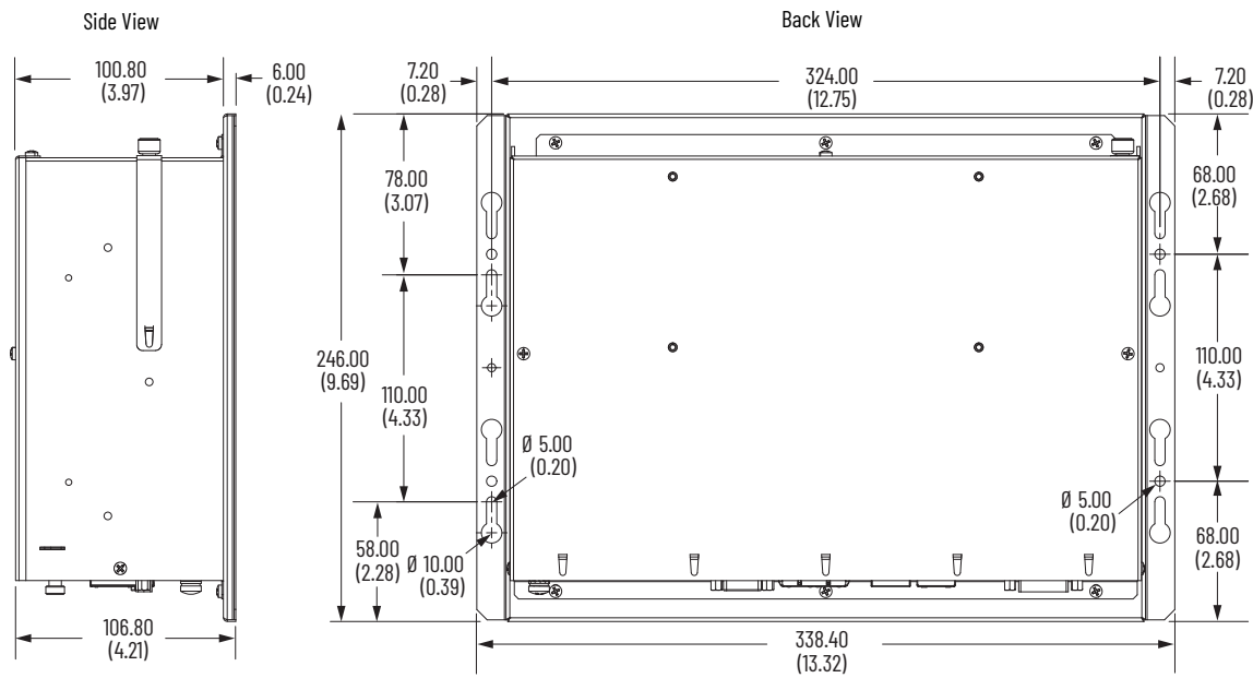
Figure 6 - 6300B-PB iClass Wall Mount Box PCs
