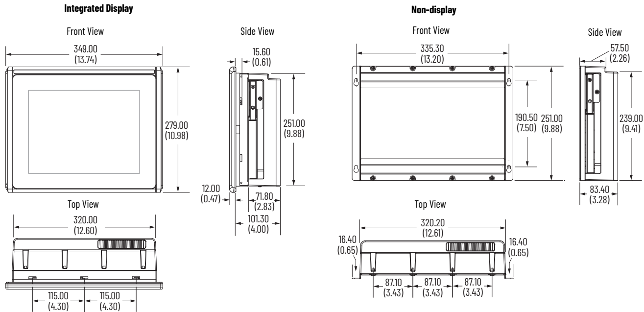
Figure 19 - Approximate Dimensions
