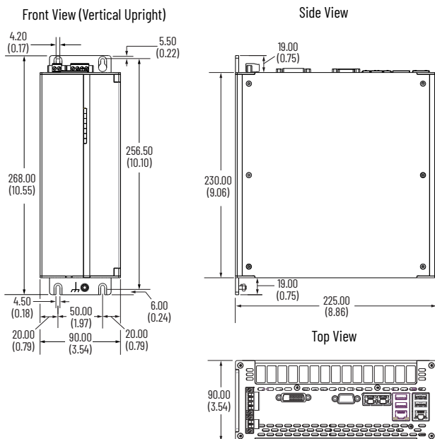
Figure 4 - 6300B-BMBDNE*, 6300B-BMBDNF*, and 6300B-BMBDNG* – S0
