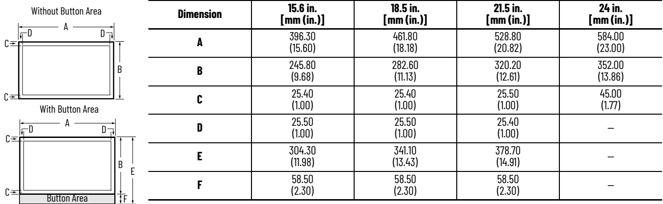
Figure 23 - 6300MA Monitors – Landscape Versions
