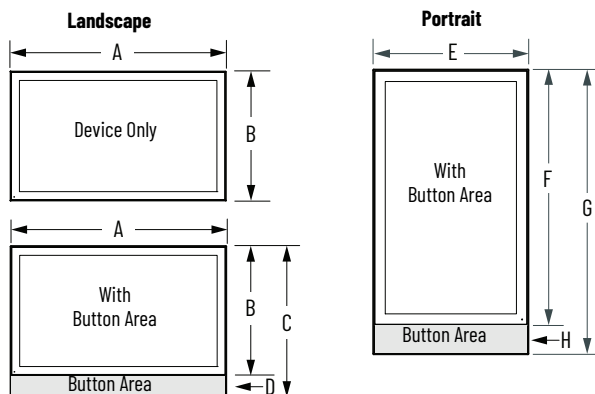
Figure 21 – Front View by LCD Size
