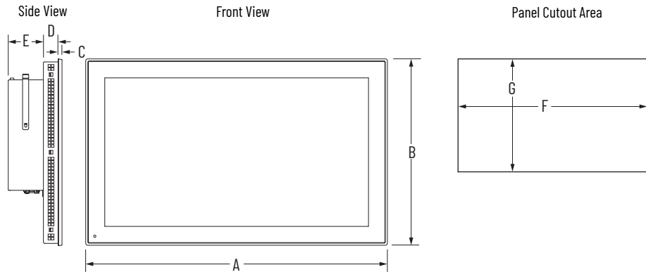
Figure 14 – 6300P Panel PC Approximate Dimensions
