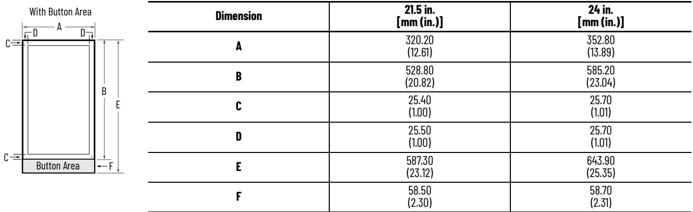
Figure 24 - 6300MA Monitors – Portrait Versions
