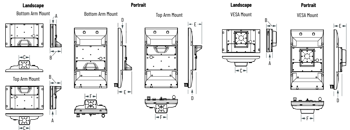
Figure 22 - Back View by LCD Size
