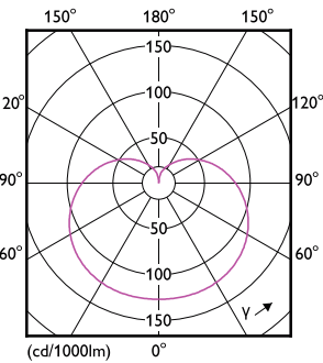
Light Distribution Diagram - 16A19/PER/927-22/P/E26/WG 6/1FB T20
