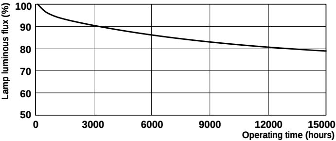
Lumen Maintenance Diagram - PL-T 57W/841/A/4P 1CT/5X10BOX ALTO
