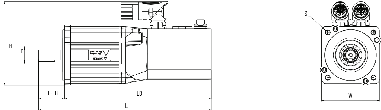
DSM Module Dimensions Table, 100 mm Frame Size
