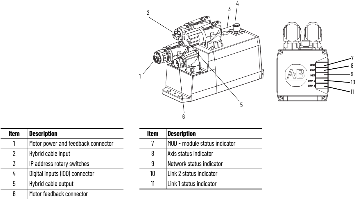
Figure 3 - Armorkinetix Distributed Servo Motor Module (DSM) Features and Indicators
