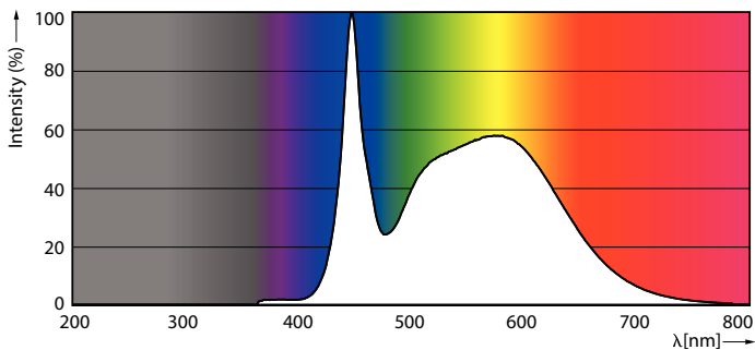
Spectral Power Distribution Colour - 40WP/LED/850/LS EX39 G3 BB 3/1
