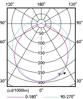
Light Distribution Diagram - 40WP/LED/850/LS EX39 G3 BB 3/1
