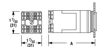
Screw Terminals with Pressure Plate Contact Block (Typical View) (1)
