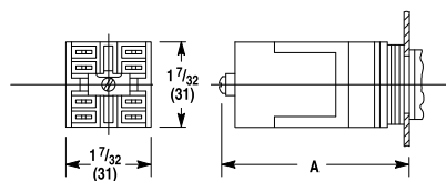
Quick Connect Terminal Contact Block (Typical View) (1)
