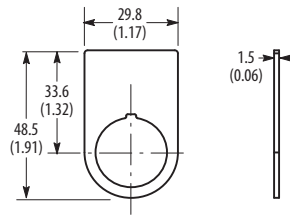
Hole Plug
