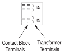
Quick Connect Terminal Contact Block (Typical View) (1)
