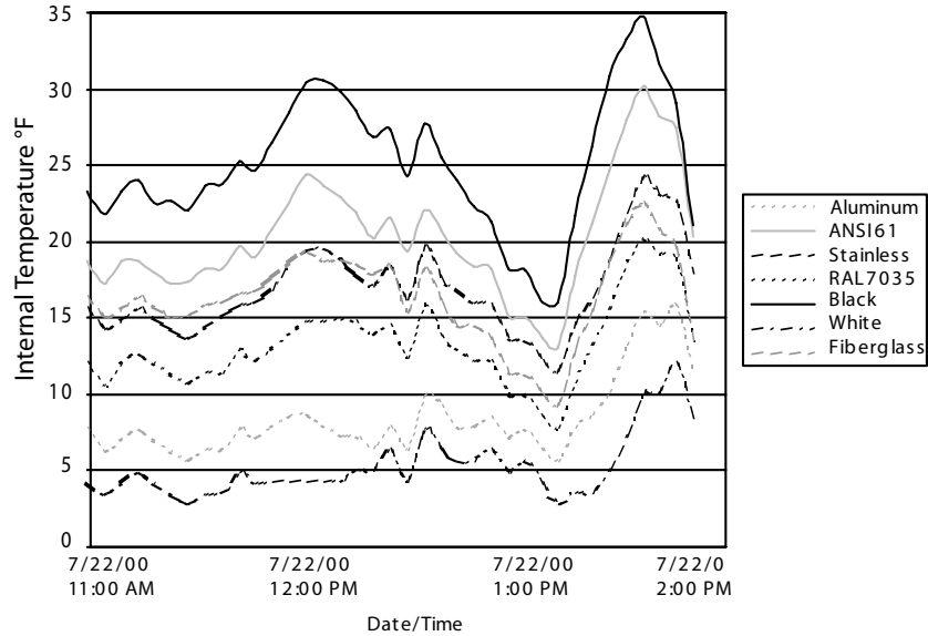
Temperature Rise Example Internal Enclosure Temperature above Outside Ambient
