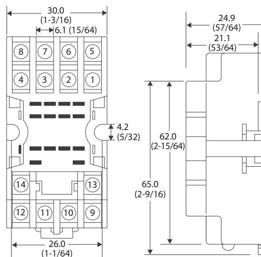
Cat. No. 700-HN128
