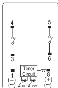
Cat. No. 700-HNK42...
