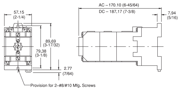
10- and 12-pole 700S-P (Captive)
