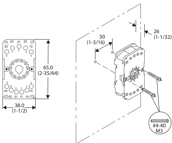
Cat. No. 700-HN101
