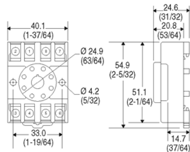
Cat. No. 700-HN125 Wire Size: 2x2.5 mm Single Wire — Up to #12 AWG Double Wire — 2x2.5 mm (#2-14...#2-20 AWG) (Either Solid or Stranded) Strip Length: 9 mm (3/8 in) — Torque: 0.8 N•m (7 lb•in)
