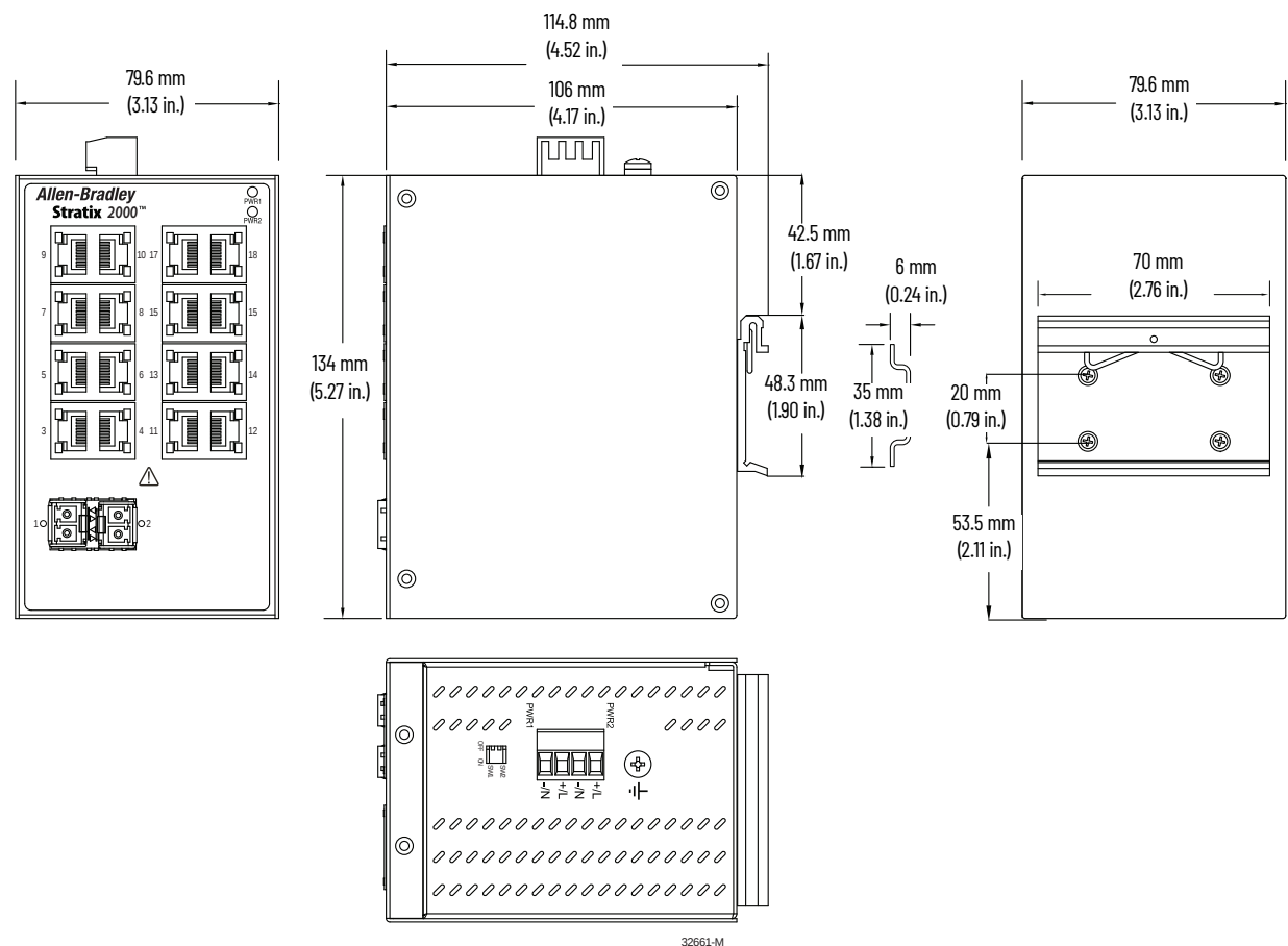
Figure 4 - 1783-US16T/B, 1783-US16T2S/B
