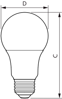
5A19/PER/927/P/E26/DIM 6/1FB T20
