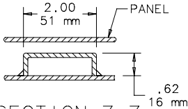
SECTION Z-Z
