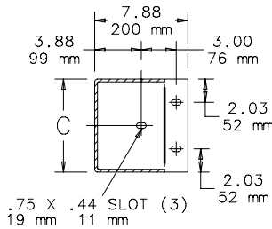
SECTION W-W
