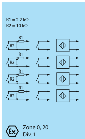
Associated Apparatus
