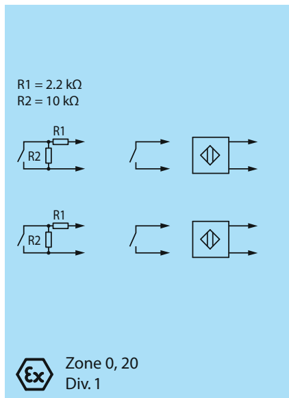
Associated Apparatus
