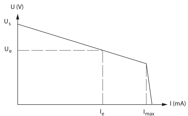
Output characteristics
