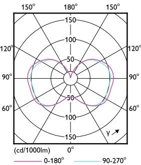
Light Distribution Diagram - 18CC/LED/840/ND E26 G2 BB 6/1
