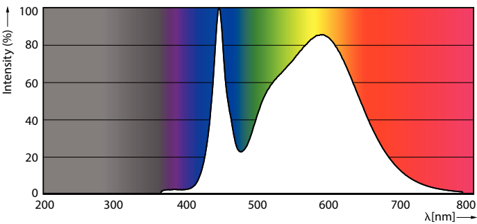
Spectral Power Distribution Colour - 18CC/LED/840/ND E26 G2 BB 6/1
