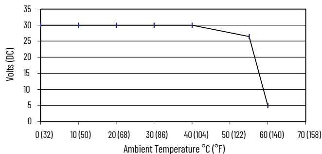
Maximum Input Voltage - 24V DC Operation
