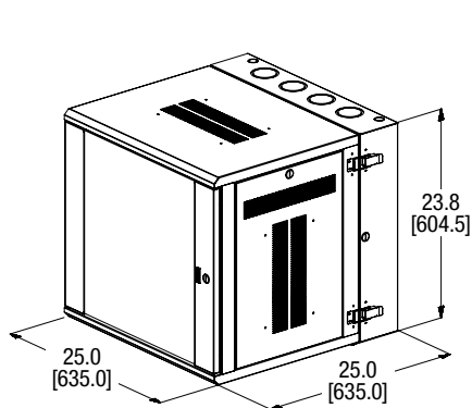
12 RU Wall Mount Cabinet
