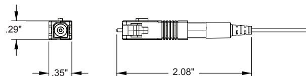
SC Connector
