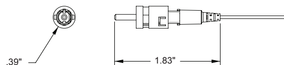
ST Connector
