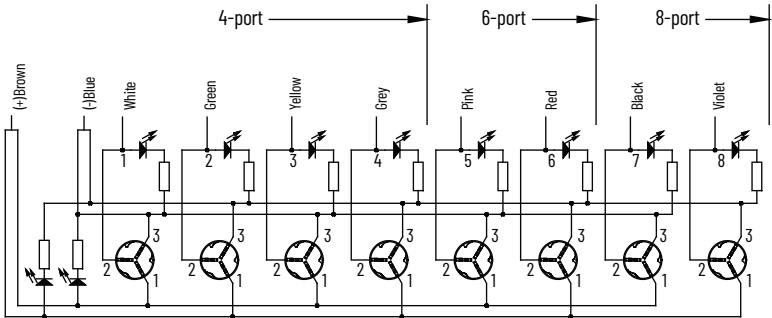
Wiring diagram shows PNP wiring. Actual units use PNP status indicator or no status indicator.
