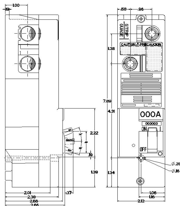
QS Breaker Dimension Drawing
