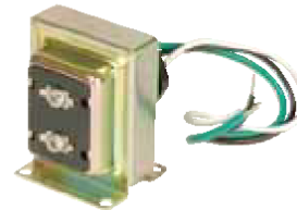
Transformer T1615 Description For Single Chime Applications with Long Wiring Distances or Dual Chime Applications, Individually Boxed Volts 16 Volt, 15VA (15 Watts)
