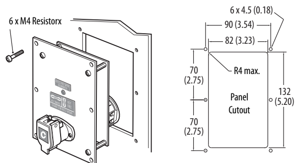
Figure 2 - Assembly
