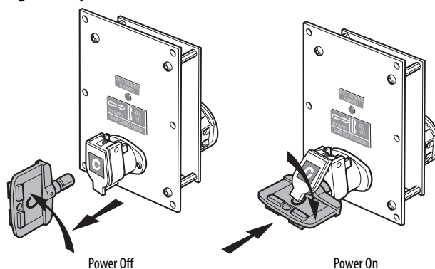
Figure 3 - Operation
