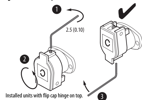
Figure 2 - Assembly
