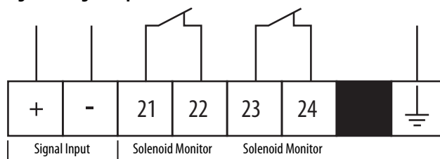
Figure 4 - Signal Input
