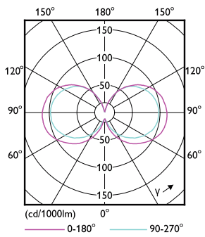
Light Distribution Diagram - 3.3BA11/PER/950/CL/G/E26/DIM 1FB T20
