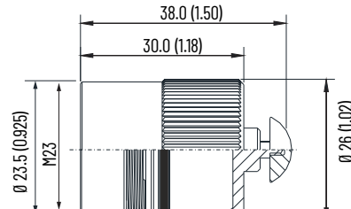
Armorkinetix DSD Power Connector Terminator - 2090-CDPT
