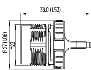
Armorkinetix DSx Hybrid Connector Output Terminator - 2090-CDHT
