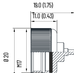
Armorkinetix DSD Feedback Connector Terminator - 2090-CDFT
