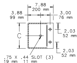
SECTION W-W
