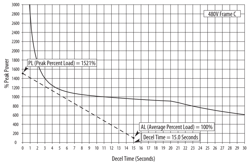
Figure 3 - Example of an Acceptable Resistor Power Curve
