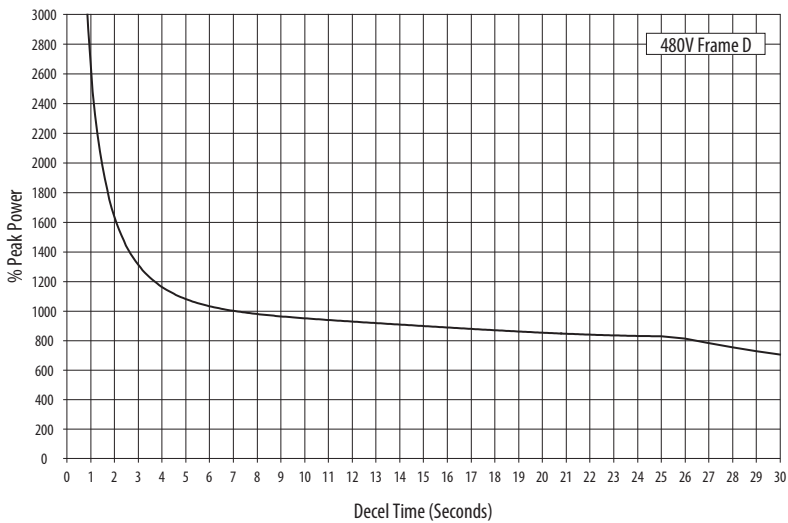
Figure 9 - PowerFlex 70 – 480 Volt, Frame D
