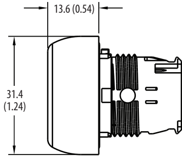
Bulletin 800FC 1-, 2-, and 3-speed Operator
