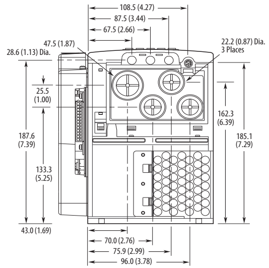
Frame 3 - All Drives except 50 HP, 480V (37 kW, 400V)
