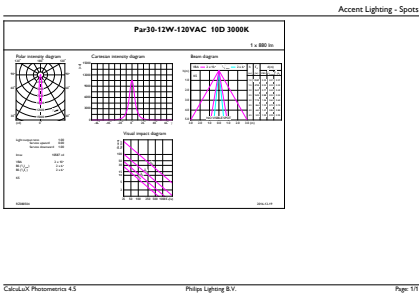
Accent Lighting Spots - 12PAR30S/EXPERTCOLOR RETAIL/S10/930/DIM
