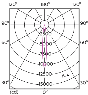
Light Distribution Diagram - 12PAR30S/EXPERTCOLOR RETAIL/S10/930/DIM
