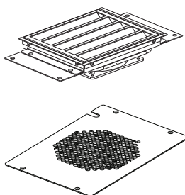
220 VAC / 50Hz fan with Shuko plug and air dam PZICFK-E
