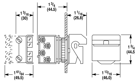
Type 4 Flip Lever Shipping Weight: 8 oz (0.14 kg)
