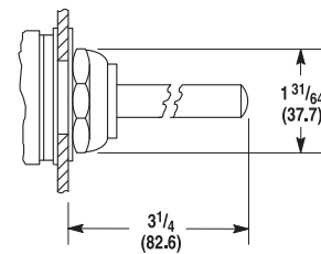
Wobble Stick Shipping Wt. 9 oz (0.25 kg)
