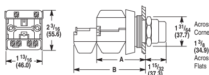
Push-to-test Pilot Light and Illuminated Push Button (Full Voltage: Incandescent, LED, Neon; and Dual Input)
