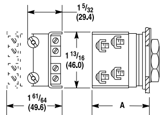
Shallow, PenTUFF, and Logic Reed Contact Blocks
