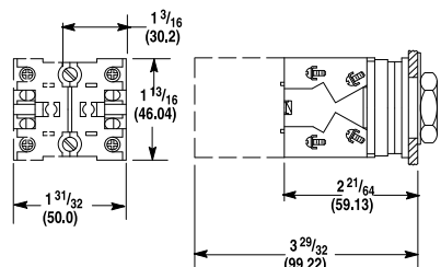
Stackable Sealed Switch Block 1.58 (40.1) Deep
