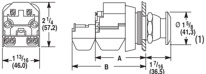
Momentary Mushroom, Push-pull and Twist or Pull Release Units (Transformer Type: Incandescent, LED; Illuminated)
