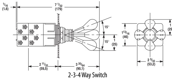
2-3-4 Way Switch Shipping Wt. with Two Contact Blocks 6 oz (0.17 kg), with 4 Contact Blocks 8-1/2 oz (0.24 kg)
