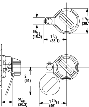
Non-illuminated Selector Switch Padlocking Adjustment
