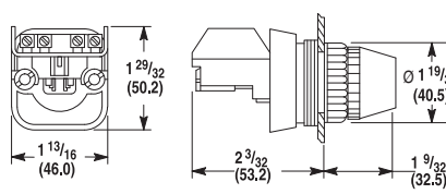
Full-voltage and Dual-input Diode Type Pilot Light (Incandescent, Neon, LED) Shipping Weight. 5 oz (0.14 kg)
