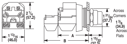
Push-to-test Pilot Light and Illuminated Push Button (Transformer Type: Incandescent, LED)
