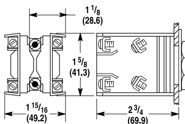
Sealed Switch Block 2 (50.8) Deep
