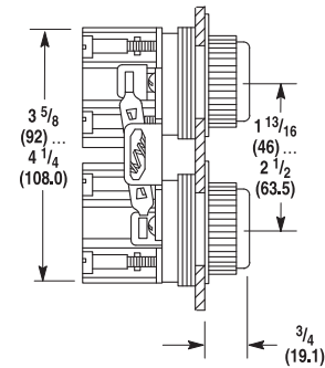
Booted Maintained Contact Push Buttons Shipping Weight: 1 lb (0.45 kg)
