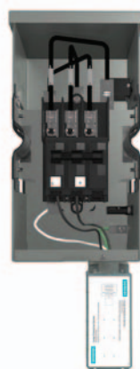
Enclosure with circuit breaker and TPS3 installed. SPD sold separately
