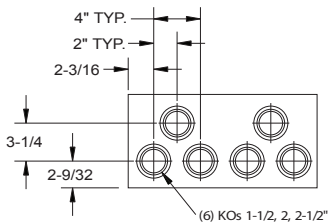
225 Amp Typical Bottom View
