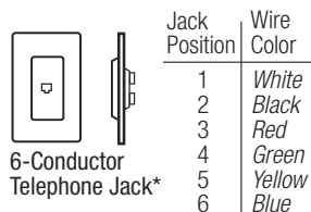
Wiring Diagram 5 Telephone Jack Wiring
