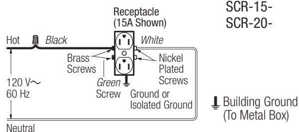
Wiring Diagram 6 Receptacle Wiring
