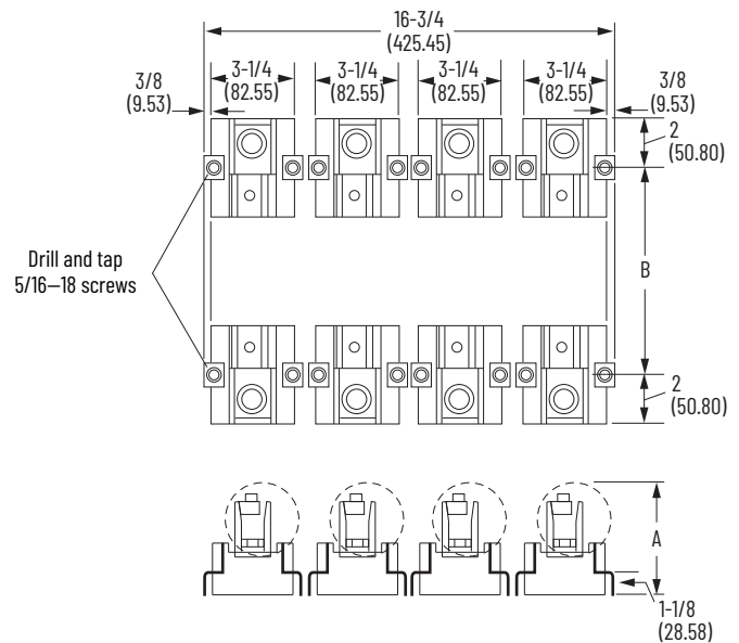
4-Pole Application Use (4) of Cat. No. 1491-N521
