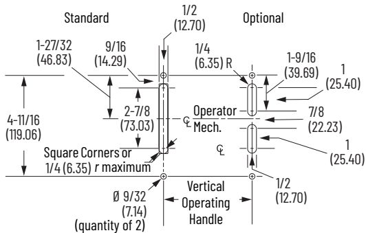
Flange Drilling
