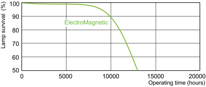
Life Expectancy Diagram - F15T8 BRIGHT WHITE/18 ALTO SL6
