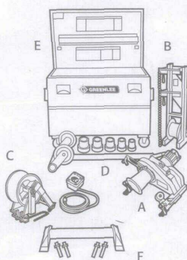
6003 Super Tugger® Cable Pulling System
