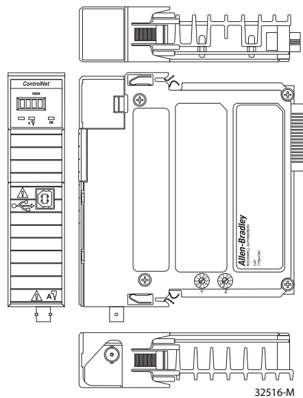
Figure 6 - 1756-CN2
