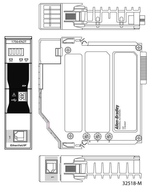
Figure 1 - 1756-EN2T
