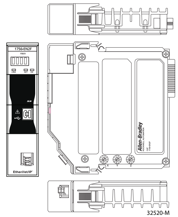
Figure 4 - 1756-EN2F
