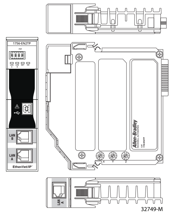
Figure 2 - 1756-EN2TP
