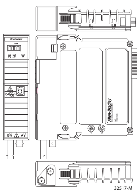
Figure 7 - 1756-CN2R
