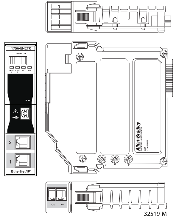
Figure 3 - 1756-EN2TR, 1756-EN3TR
