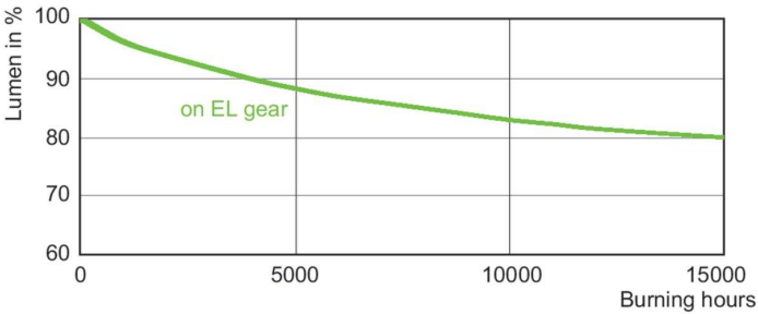
Lumen Maintenance Diagram - MASTERColor CDM-T Elite 35W/930 G12 1CT
