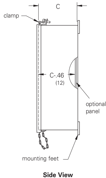
Cover Clamp Layout
