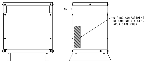
Enclosure Style 2 - Ventilated 11 kVA to 112.5 kVA
