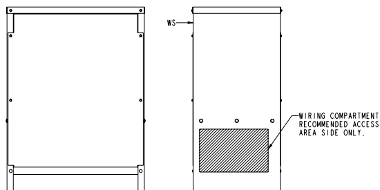
Enclosure Design Style 1 - Ventilated 118 kVA to 500 kVA
