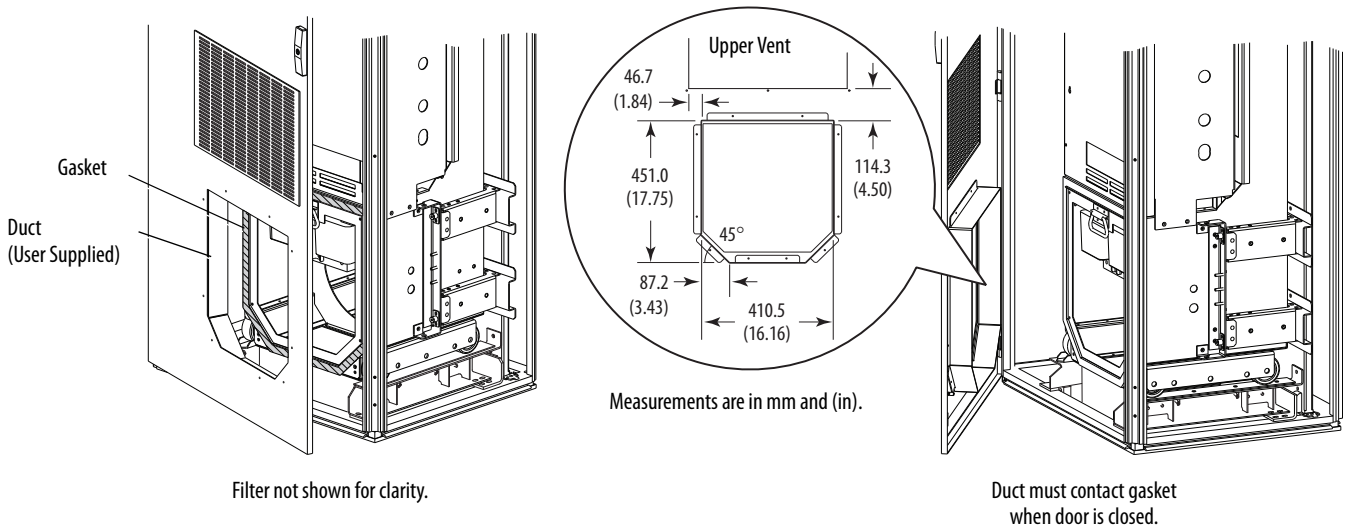
Figure 2 - Intake Duct Details
