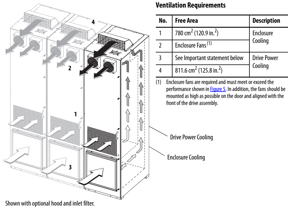
Figure 1 - Dual Airflow System
