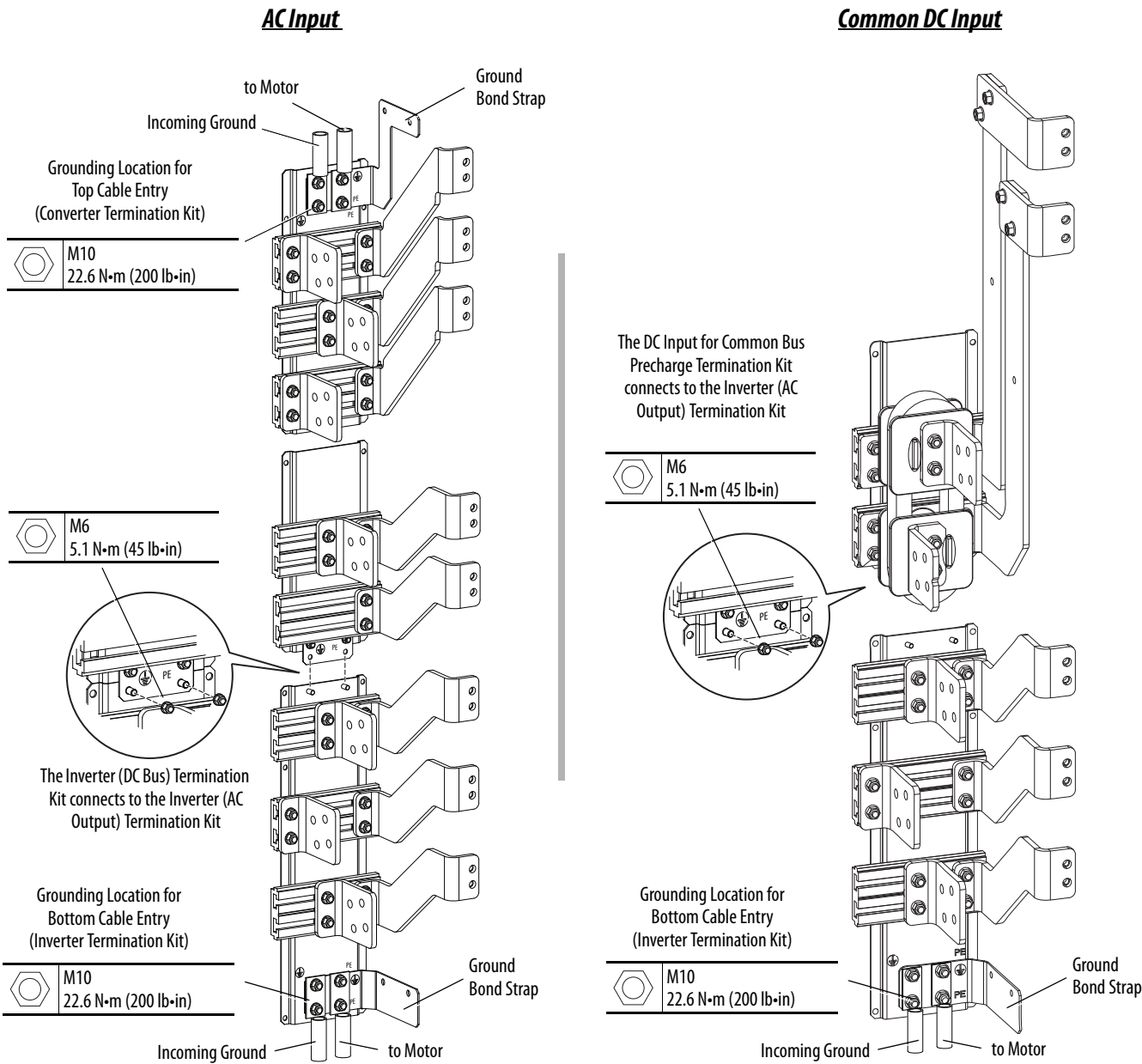
Figure 7 - Drive Grounding
