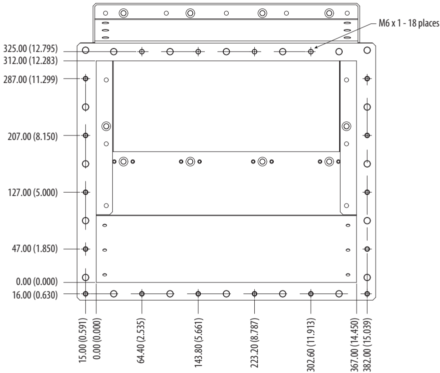
Figure 9 - Bottom Inlet Ducting Kit Dimensions
