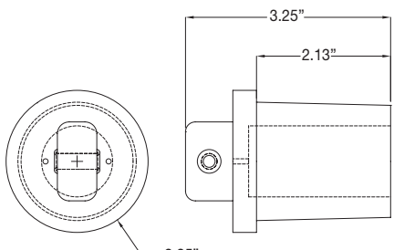
Male cap
