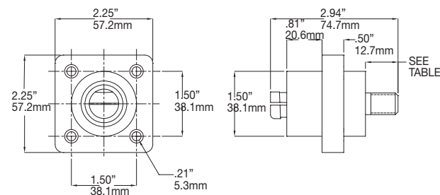
Male receptacle
