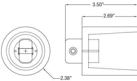
Female cap
